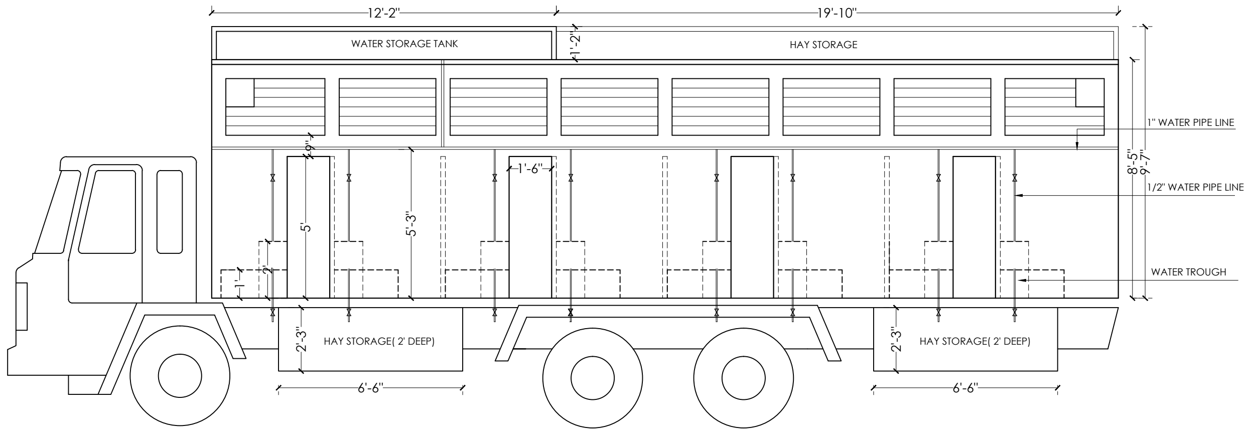
RIGHT SIDE ELEVATION WITH CARRIER
